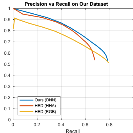
PR curve on our new dataset.
