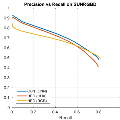
PR curve on SUNRGBD.
