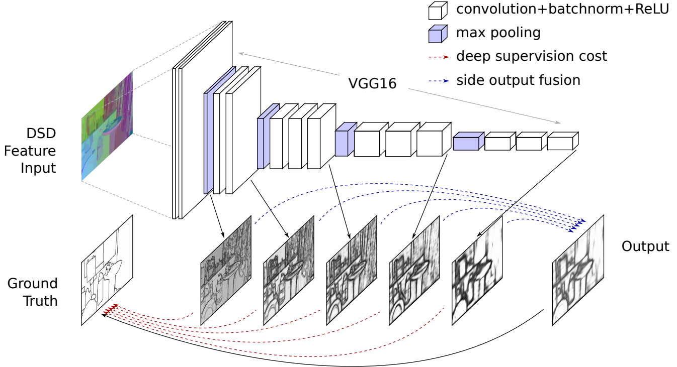
Figure 3. An overview of our edge detection system. Our DSD encoding of the depth map is the input to fully convolutional VGG16 network with deep supervision, as in [29]. We add a batch normalization layer after every convolutional layer to speed up convergence.
